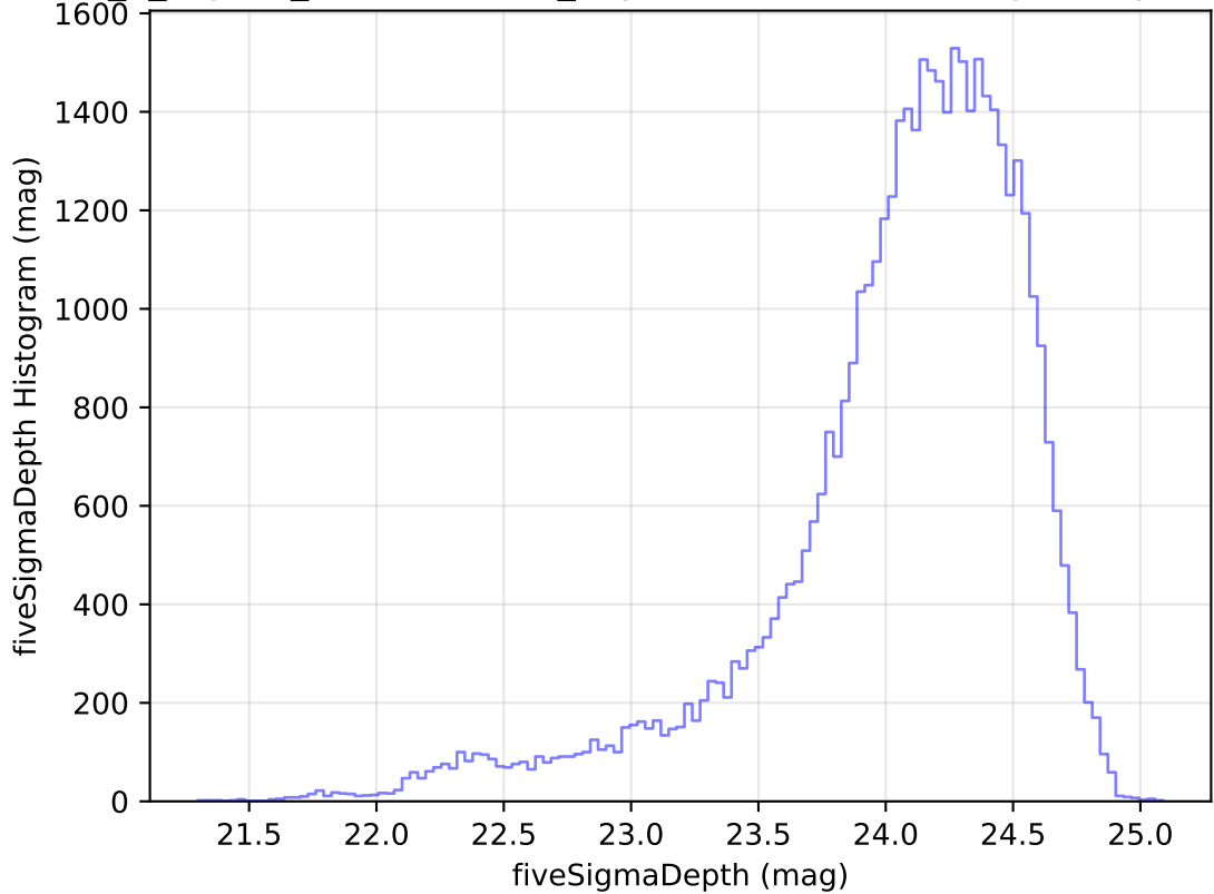
internal_u_expt60_nscale1.2v3.4_10yrs Yr 1 r band: fiveSigmaDepth Histogram
