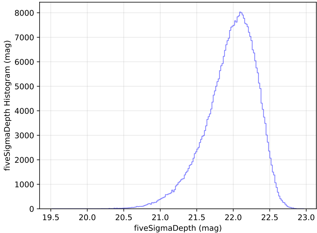
internal_u_expt60_nscale1.2v3.4_10yrs WFD y band: fiveSigmaDepth Histogram
