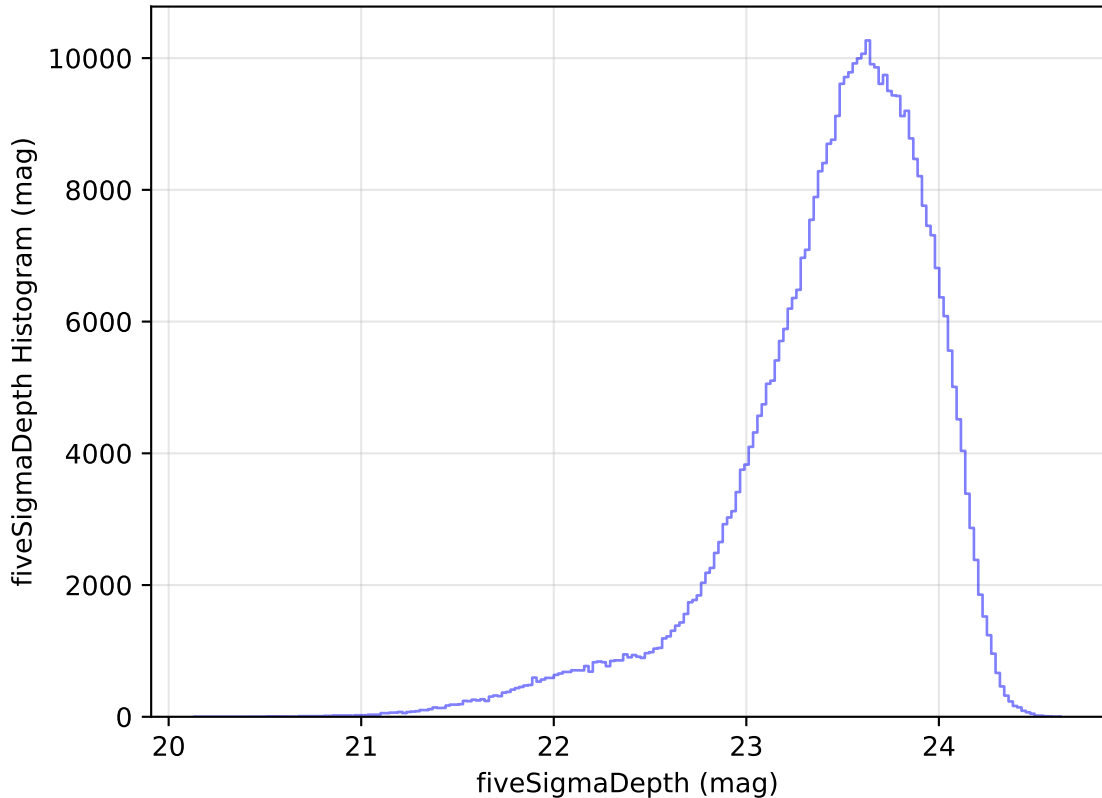
internal_u_expt60_nscale1.2v3.4_10yrs WFD i band: fiveSigmaDepth Histogram
