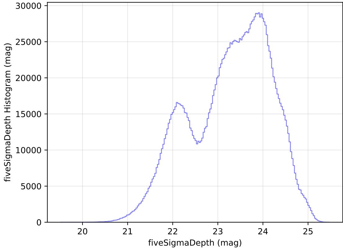
internal_u_expt60_nscale1.2v3.4_10yrs WFD all bands: fiveSigmaDepth Histogram
