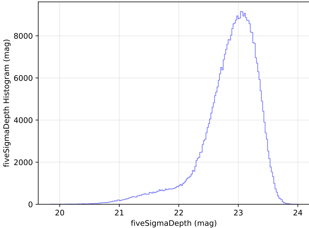
internal_u_expt60_nscale1.2v3.4_10yrs All sky z band: fiveSigmaDepth Histogram
