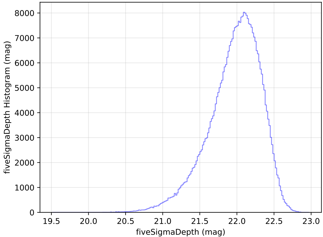
internal_u_expt60_nscale1.2v3.4_10yrs All sky y band: fiveSigmaDepth Histogram
