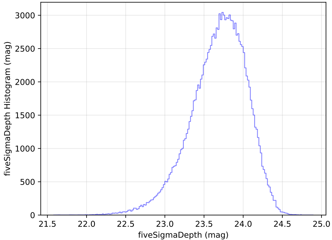
internal_u_expt60_nscale1.2v3.4_10yrs All sky u band: fiveSigmaDepth Histogram
