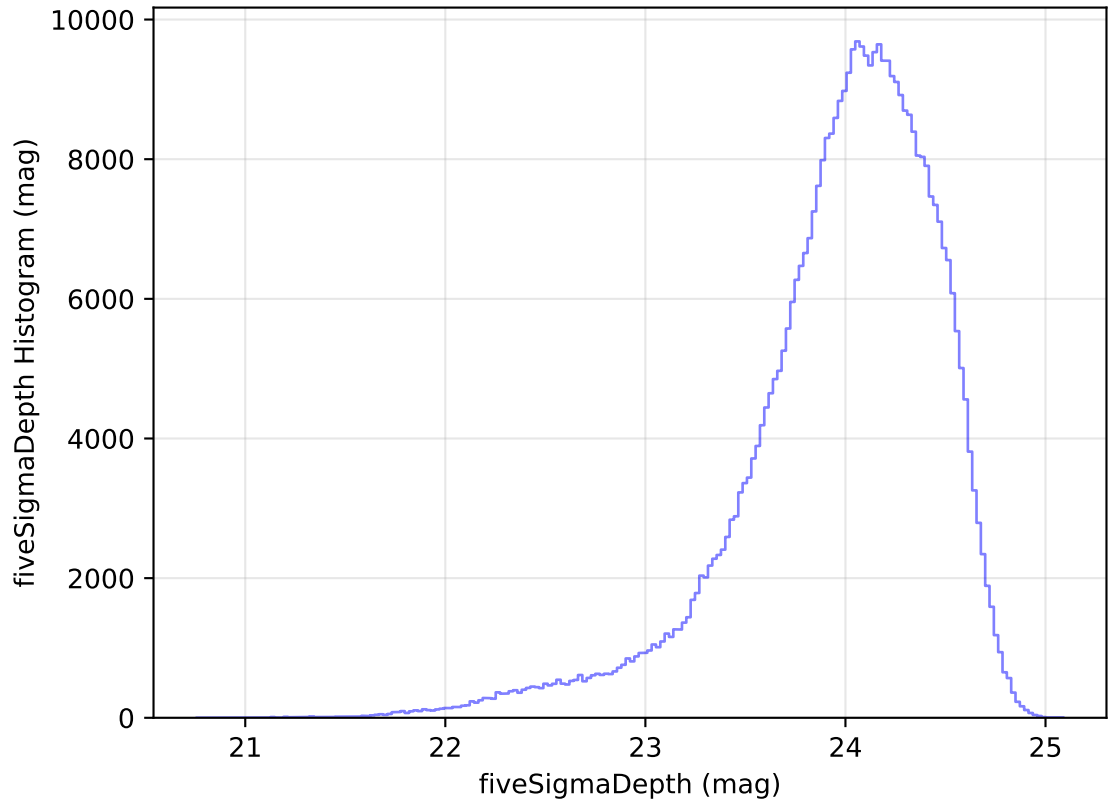
internal_u_expt60_nscale1.2v3.4_10yrs All sky r band: fiveSigmaDepth Histogram
