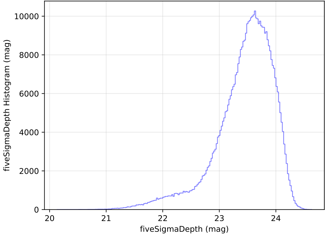
internal_u_expt60_nscale1.2v3.4_10yrs All sky i band: fiveSigmaDepth Histogram
