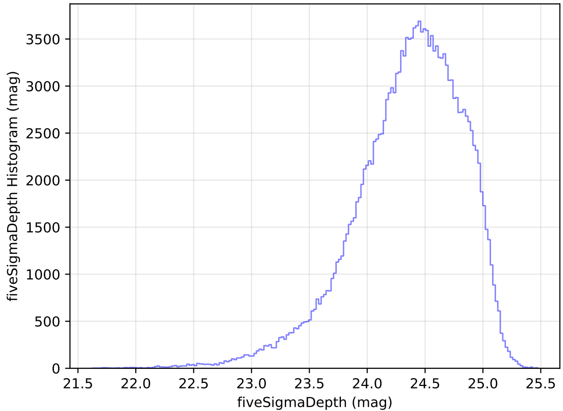
internal_u_expt60_nscale1.2v3.4_10yrs All sky g band: fiveSigmaDepth Histogram
