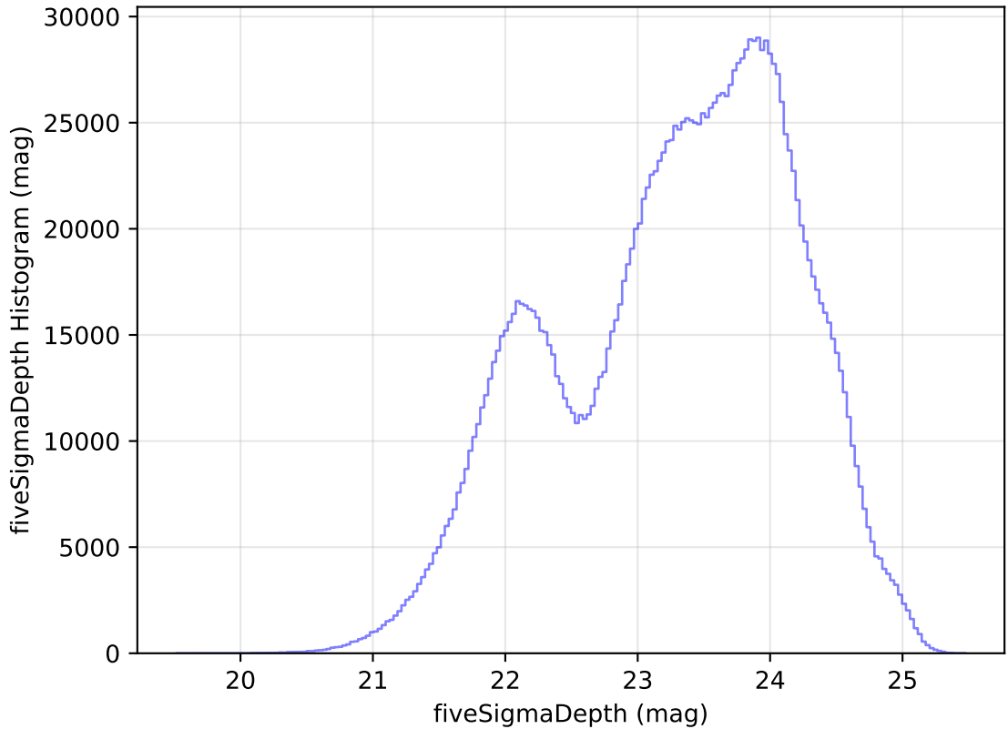
internal_u_expt60_nscale1.2v3.4_10yrs All sky all bands: fiveSigmaDepth Histogram
