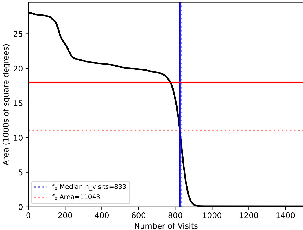
internal_u_expt60_nscale1.2v3.4_10yrs All sky: f0
