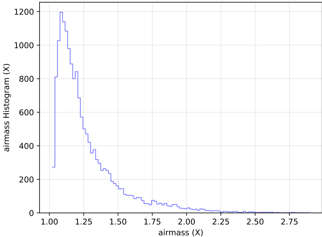
internal_u_expt60_nscale1.2v3.4_10yrs Yr 1 u band: airmass Histogram
