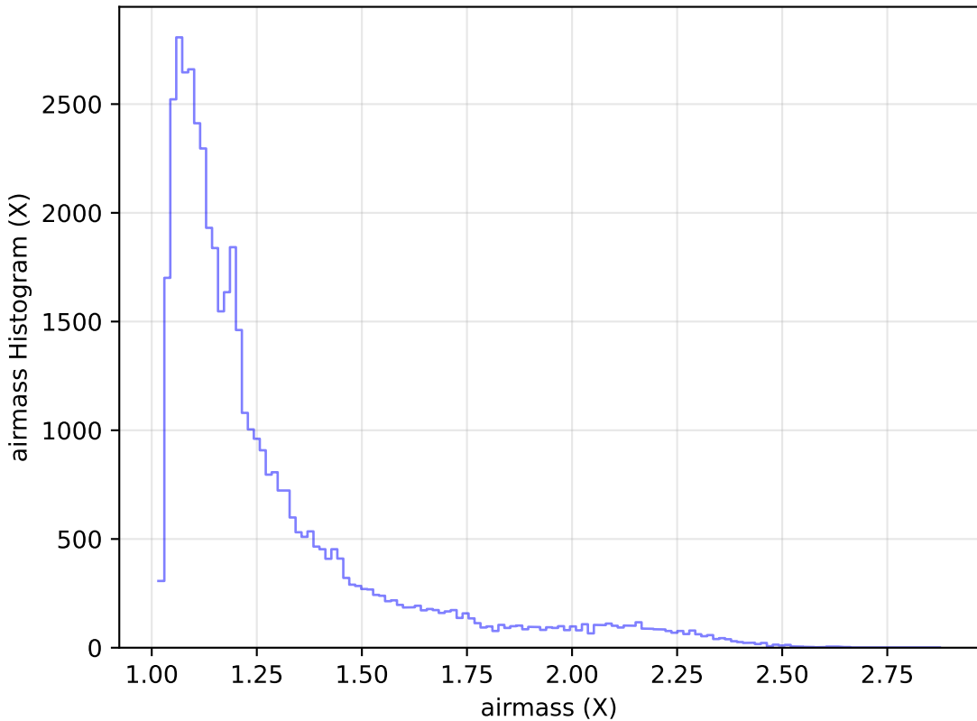
internal_u_expt60_nscale1.2v3.4_10yrs Yr 1 r band: airmass Histogram
