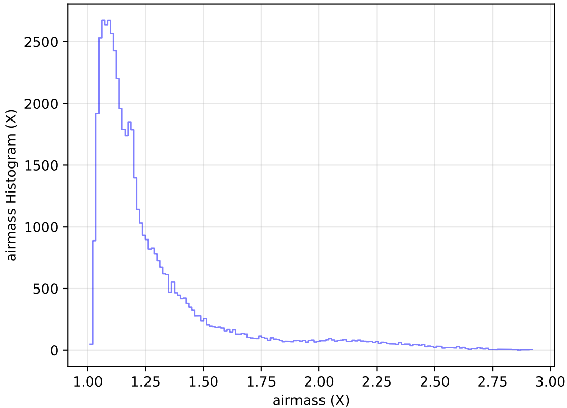
internal_u_expt60_nscale1.2v3.4_10yrs Yr 1 i band: airmass Histogram
