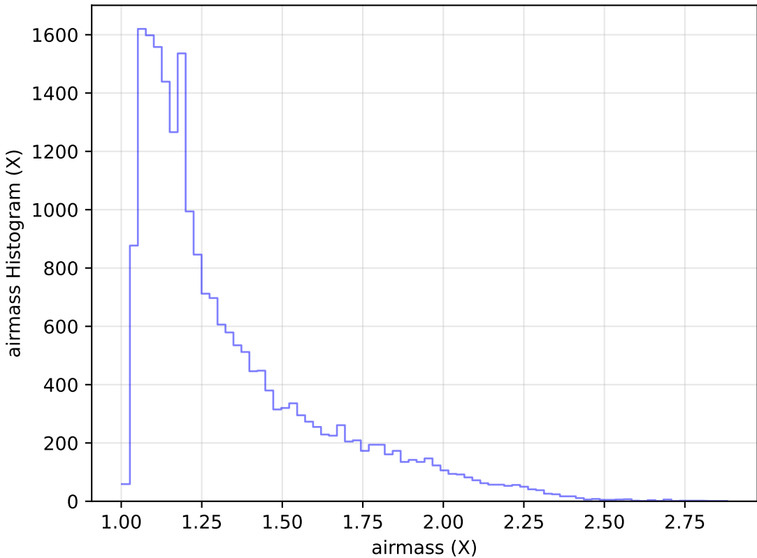
internal_u_expt60_nscale1.2v3.4_10yrs Yr 1 g band: airmass Histogram
