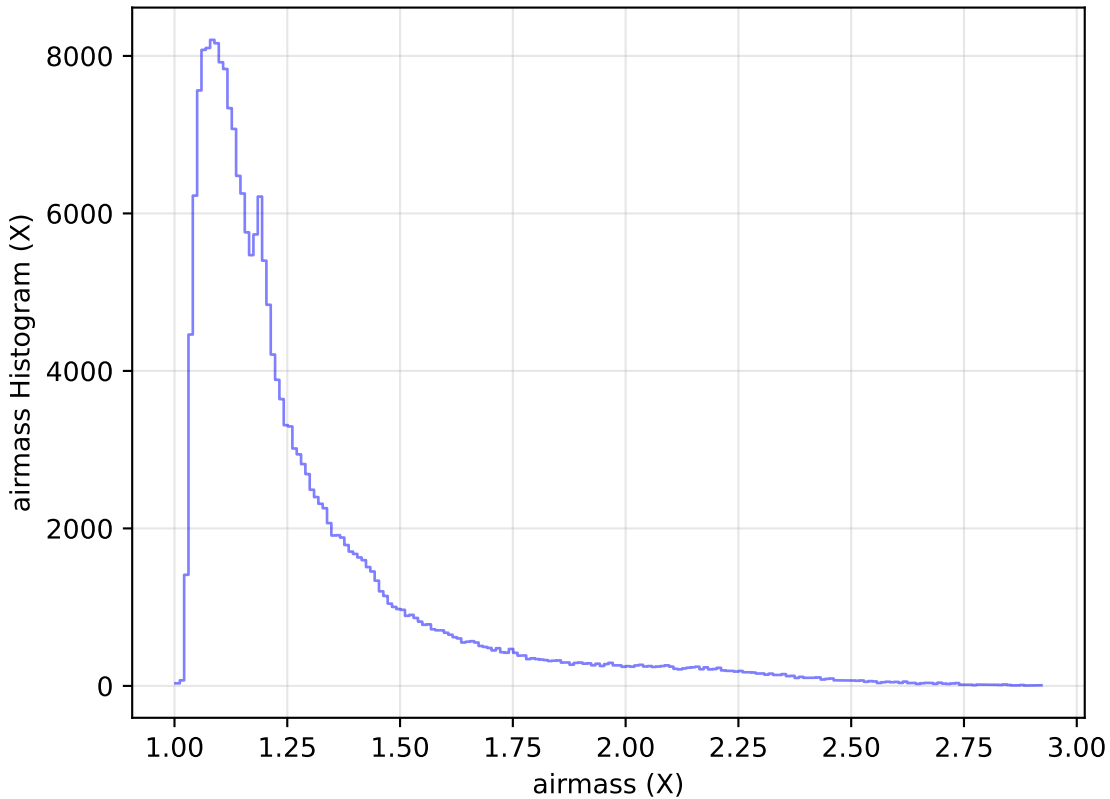
internal_u_expt60_nscale1.2v3.4_10yrs Yr 1 all bands: airmass Histogram
