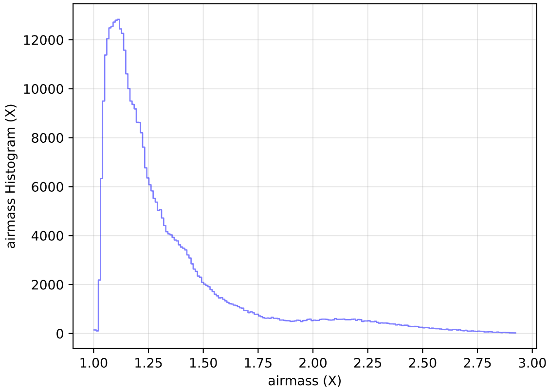
internal_u_expt60_nscale1.2v3.4_10yrs WFD z band: airmass Histogram
