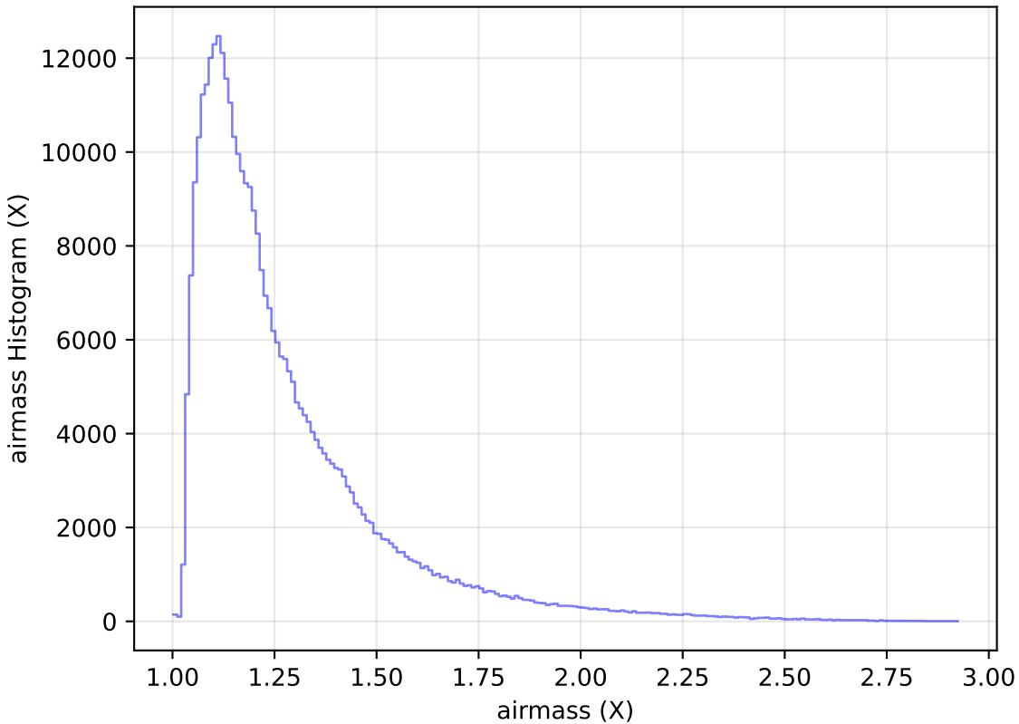
internal_u_expt60_nscale1.2v3.4_10yrs WFD y band: airmass Histogram
