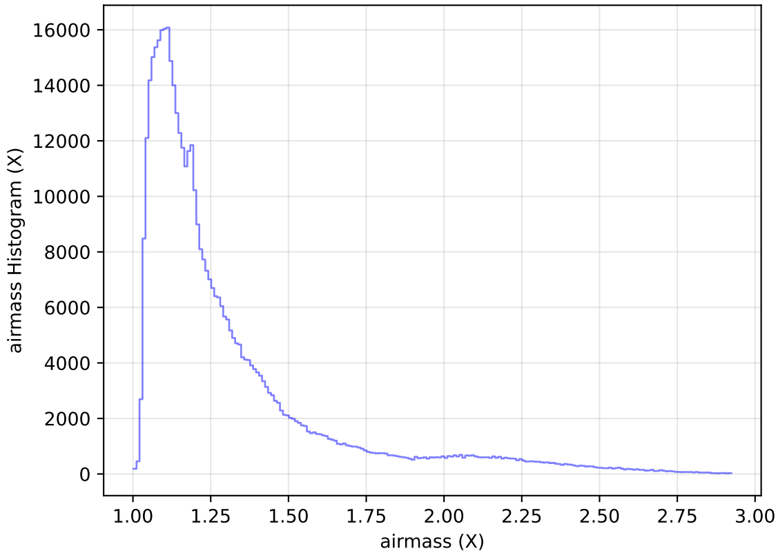
internal_u_expt60_nscale1.2v3.4_10yrs WFD i band: airmass Histogram
