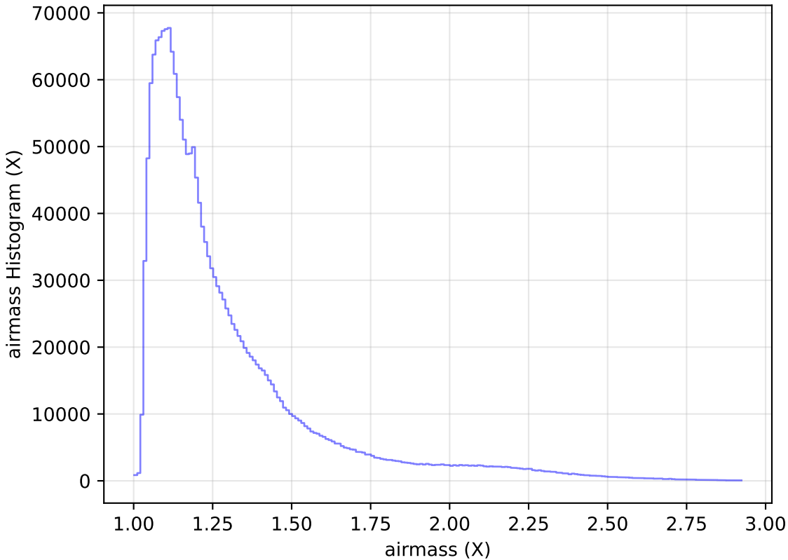
internal_u_expt60_nscale1.2v3.4_10yrs WFD all bands: airmass Histogram
