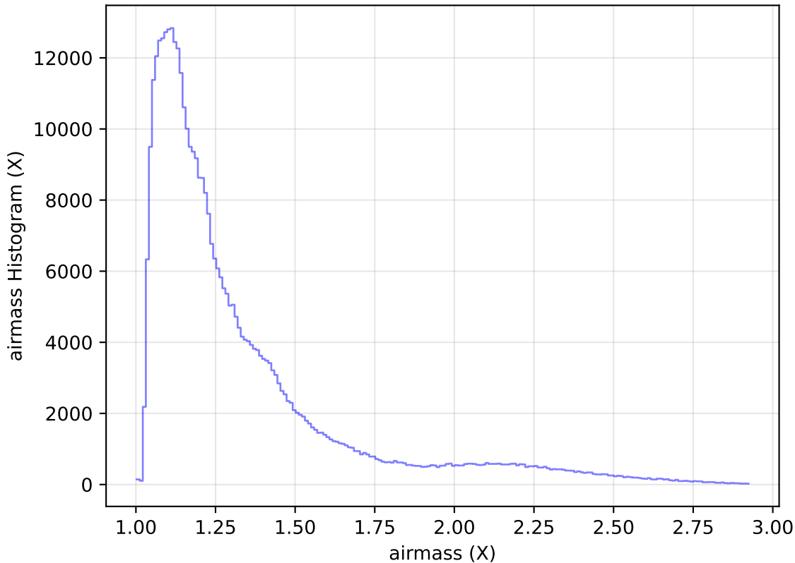
internal_u_expt60_nscale1.2v3.4_10yrs All sky z band: airmass Histogram
