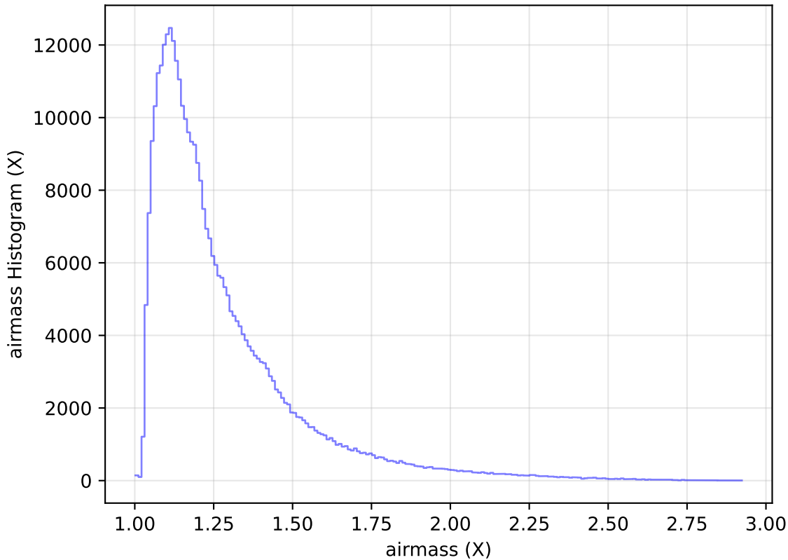
internal_u_expt60_nscale1.2v3.4_10yrs All sky y band: airmass Histogram
