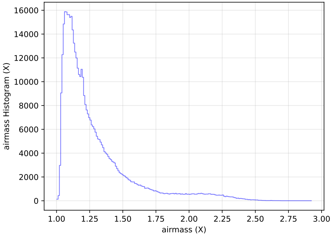
internal_u_expt60_nscale1.2v3.4_10yrs All sky r band: airmass Histogram
