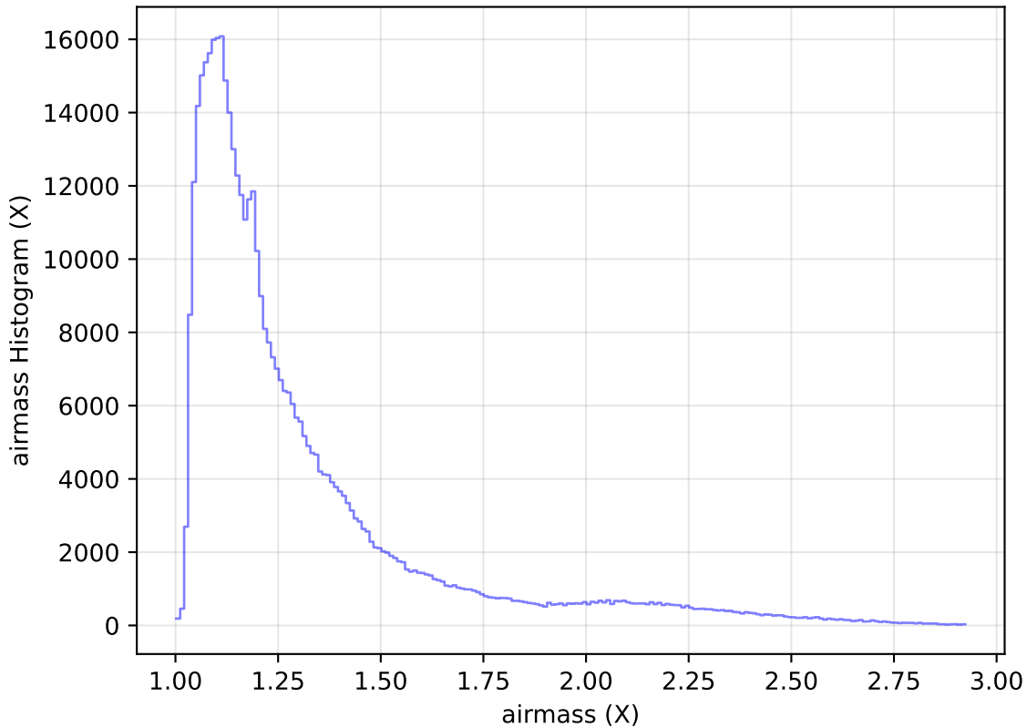
internal_u_expt60_nscale1.2v3.4_10yrs All sky i band: airmass Histogram
