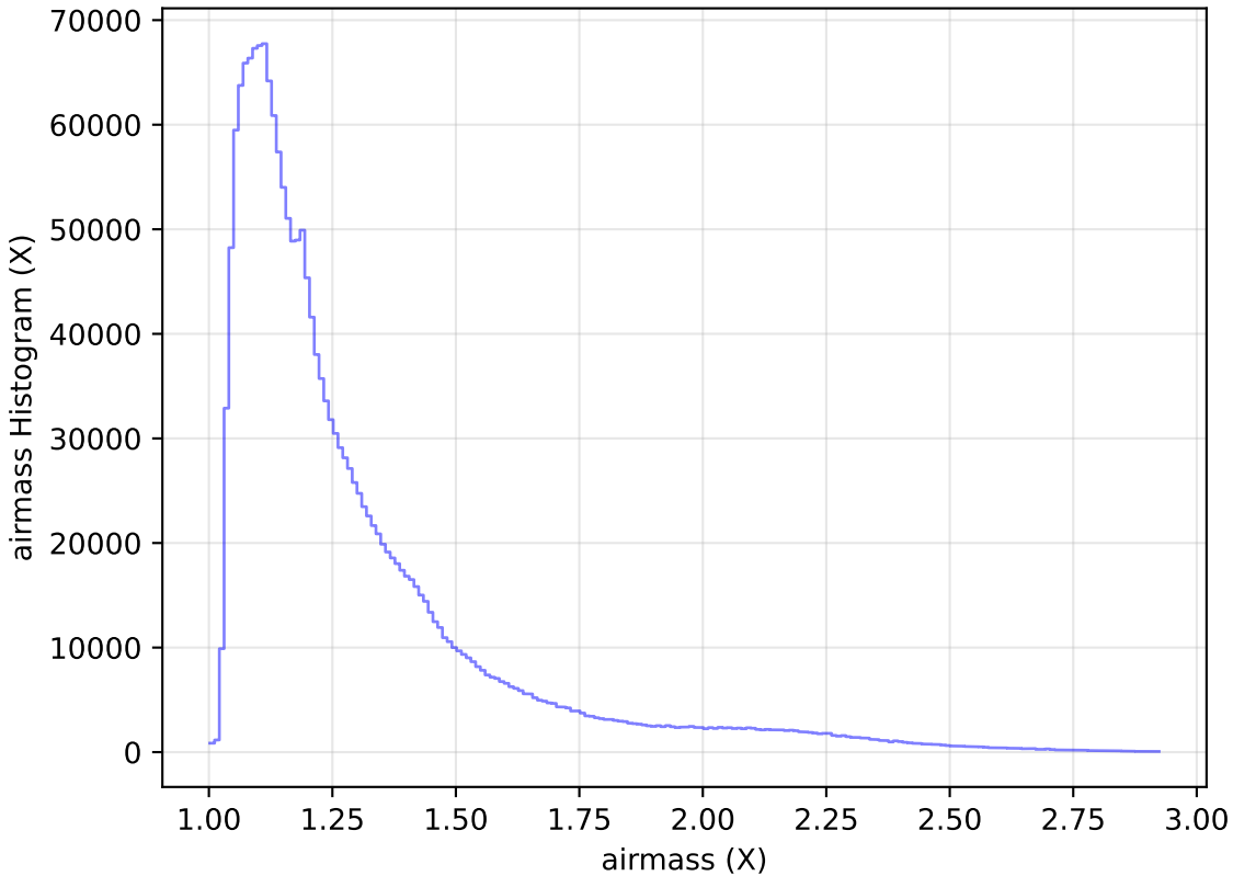
internal_u_expt60_nscale1.2v3.4_10yrs All sky all bands: airmass Histogram
