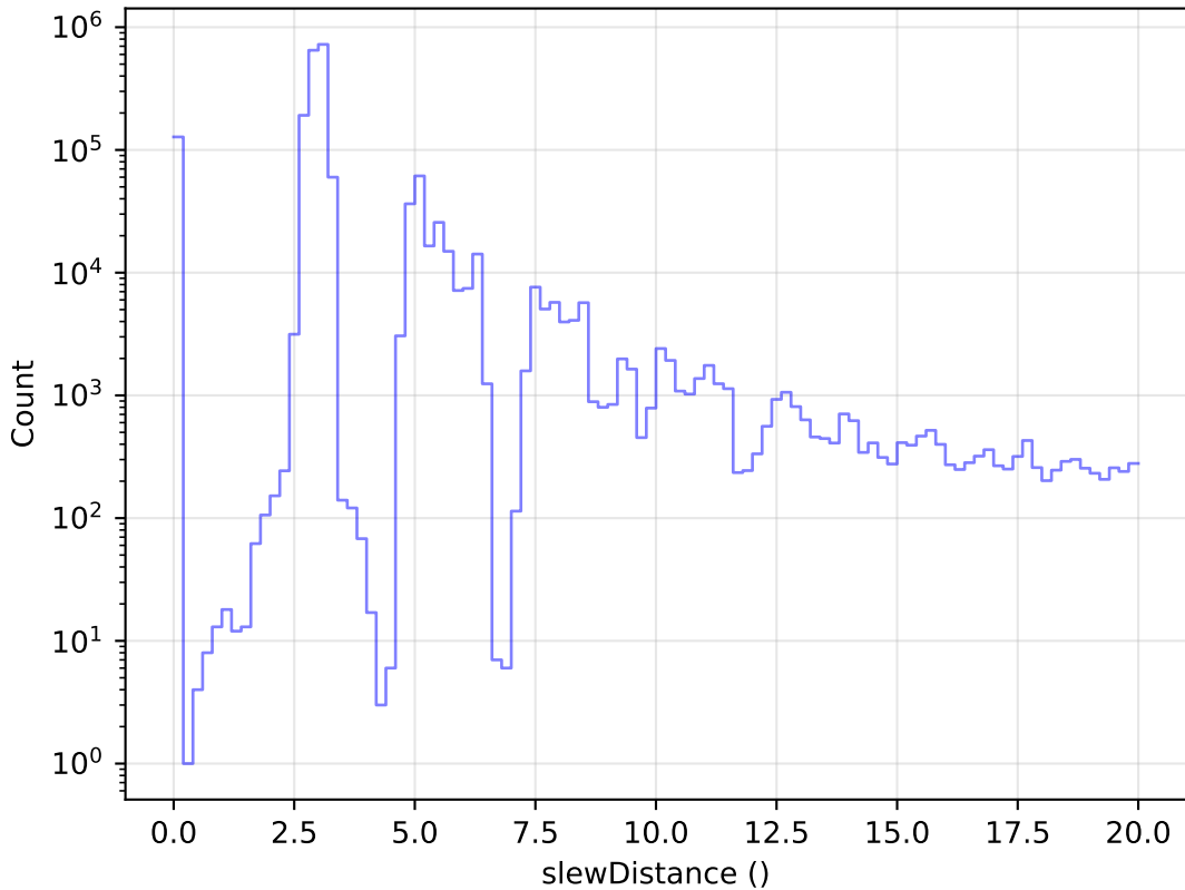
internal_u_expt60_nscale1.2v3.4_10yrs All visits: Zoom Slew Distance Histogram
