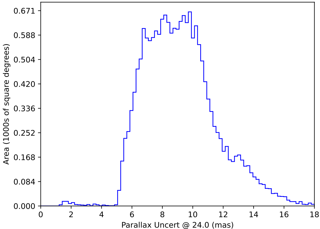
internal_u_expt60_nscale1.2v3.4_10yrs WFD: Parallax Uncert @ 24.0
