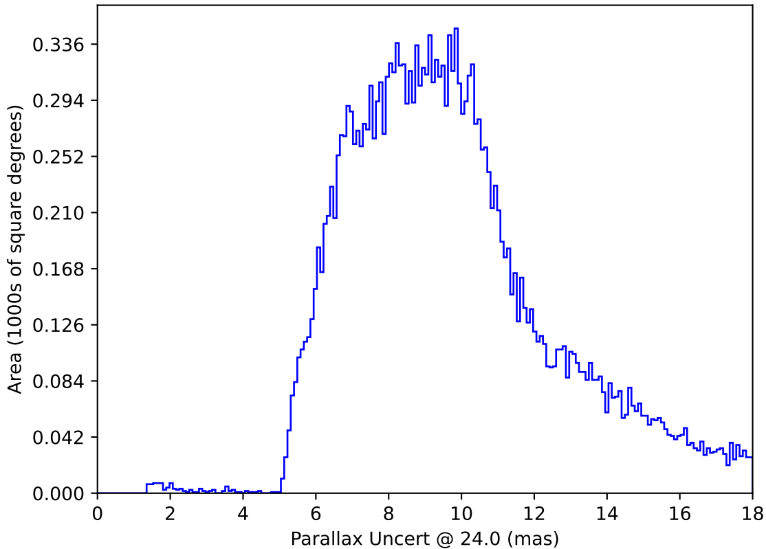
internal_u_expt60_nscale1.2v3.4_10yrs All sky: Parallax Uncert @ 24.0
