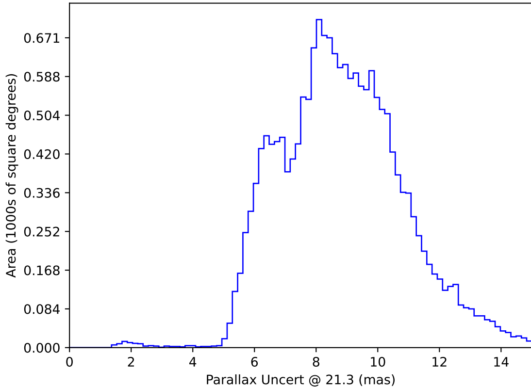
internal_u_expt60_nscale1.2v3.4_10yrs WFD y band only: Parallax Uncert @ 21.3
