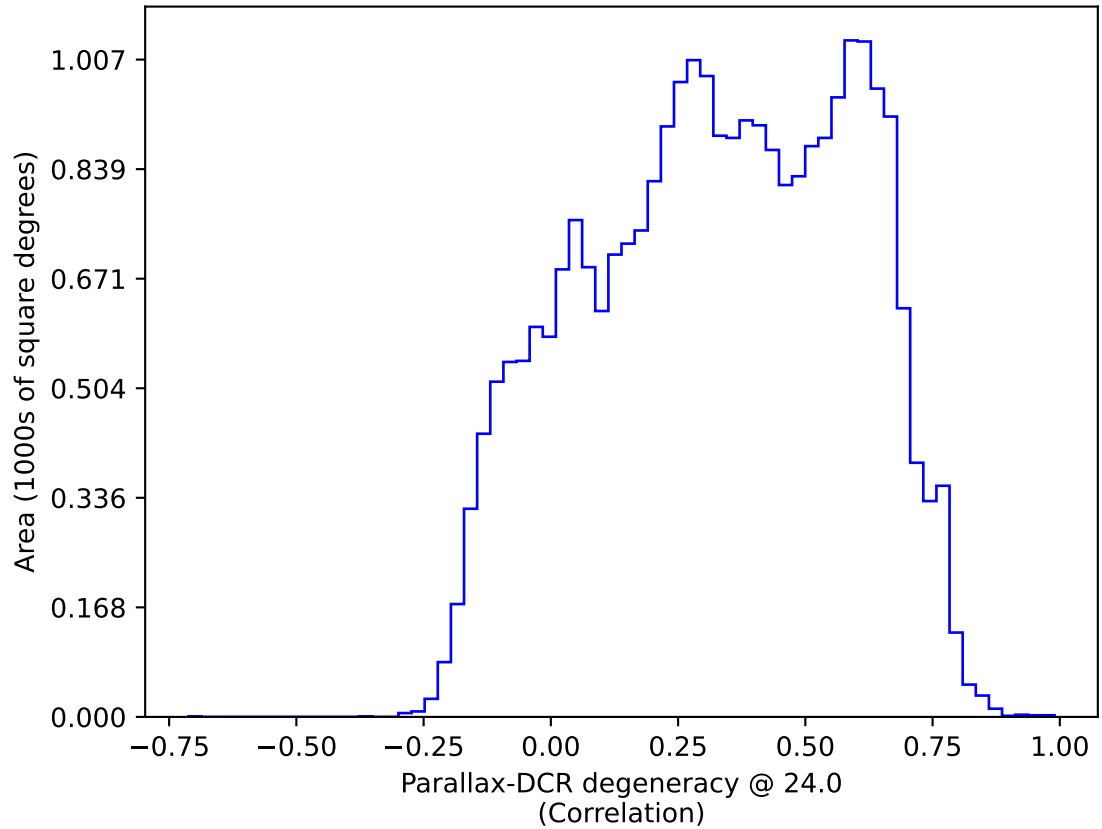
internal_u_expt60_nscale1.2v3.4_10yrs All sky: Parallax-DCR degeneracy @ 24.0
