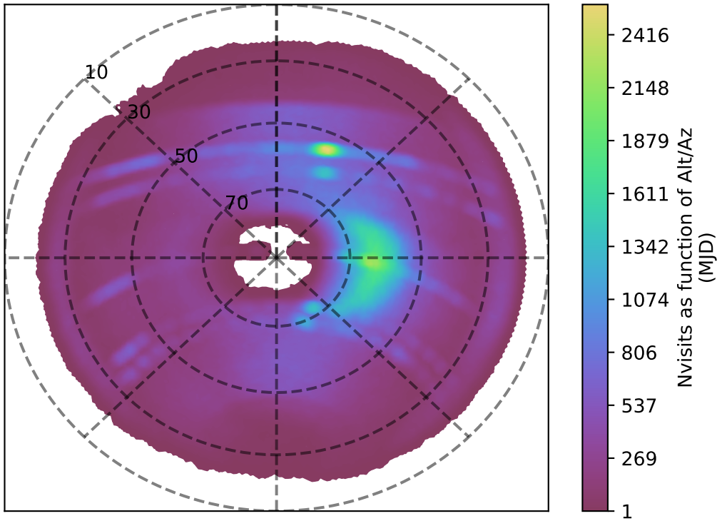
internal_u_expt60_nscale1.2v3.4_10yrs z band: Nvisits as function of Alt/Az
