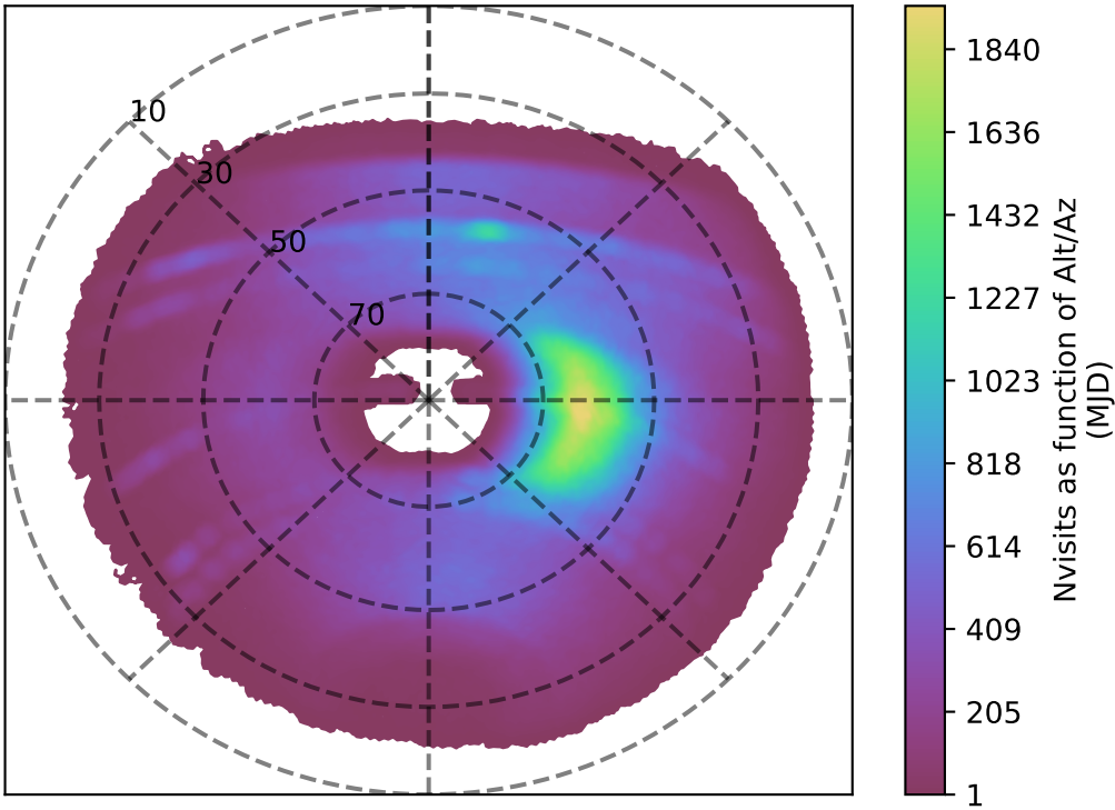
internal_u_expt60_nscale1.2v3.4_10yrs y band: Nvisits as function of Alt/Az
