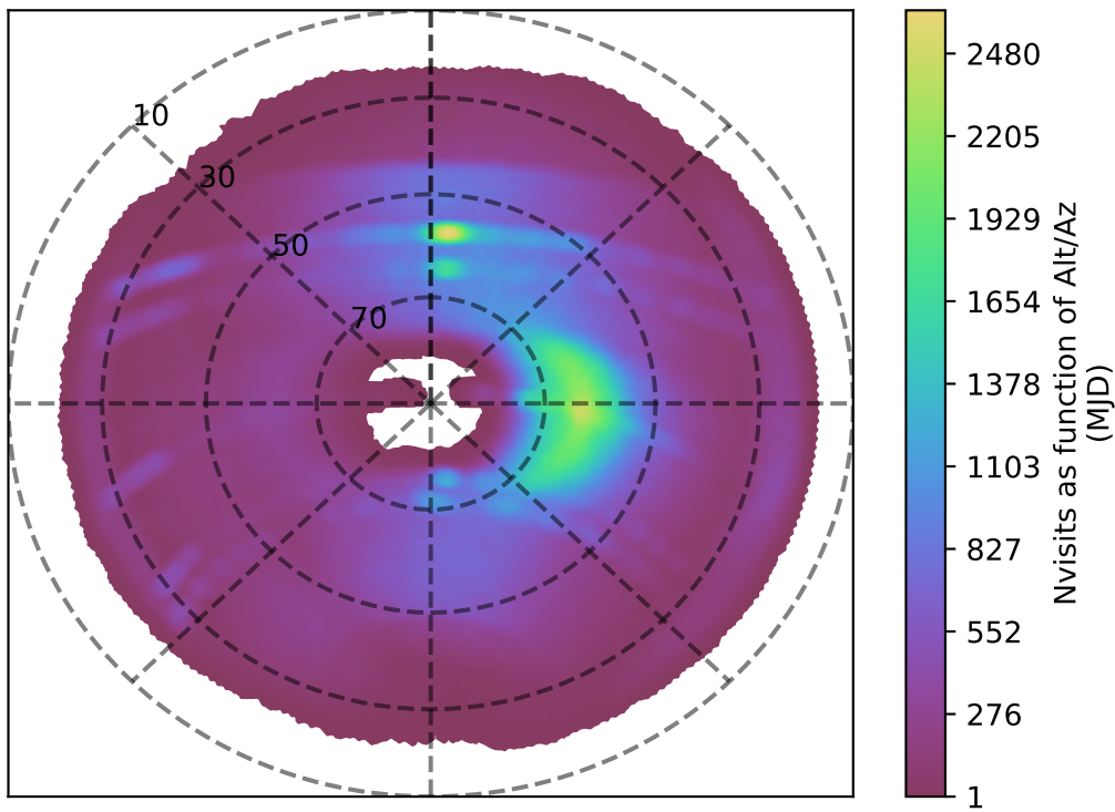
internal_u_expt60_nscale1.2v3.4_10yrs i band: Nvisits as function of Alt/Az
