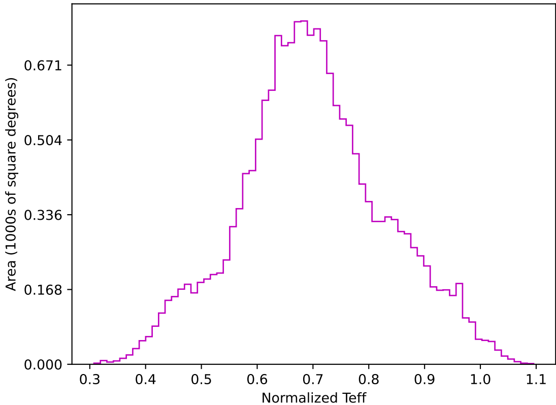
internal_u_expt60_nscale1.2v3.4_10yrs WFD z band: Normalized Teff
