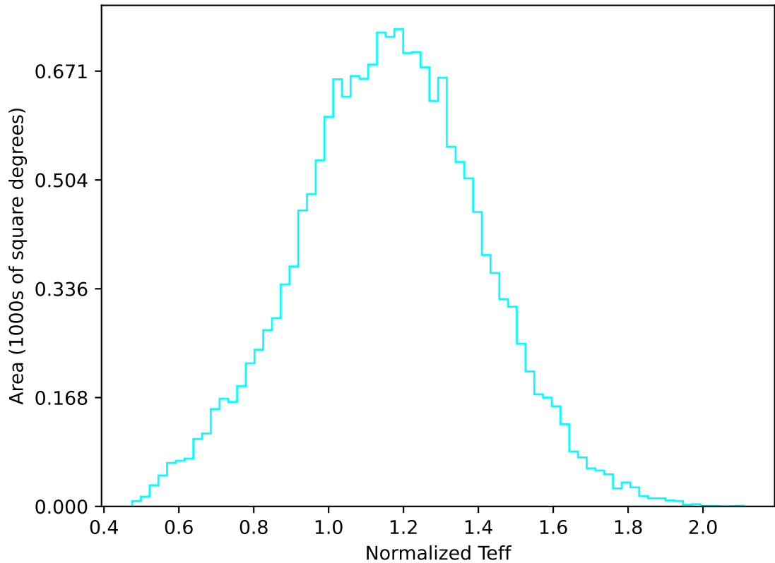
internal_u_expt60_nscale1.2v3.4_10yrs WFD u band: Normalized Teff
