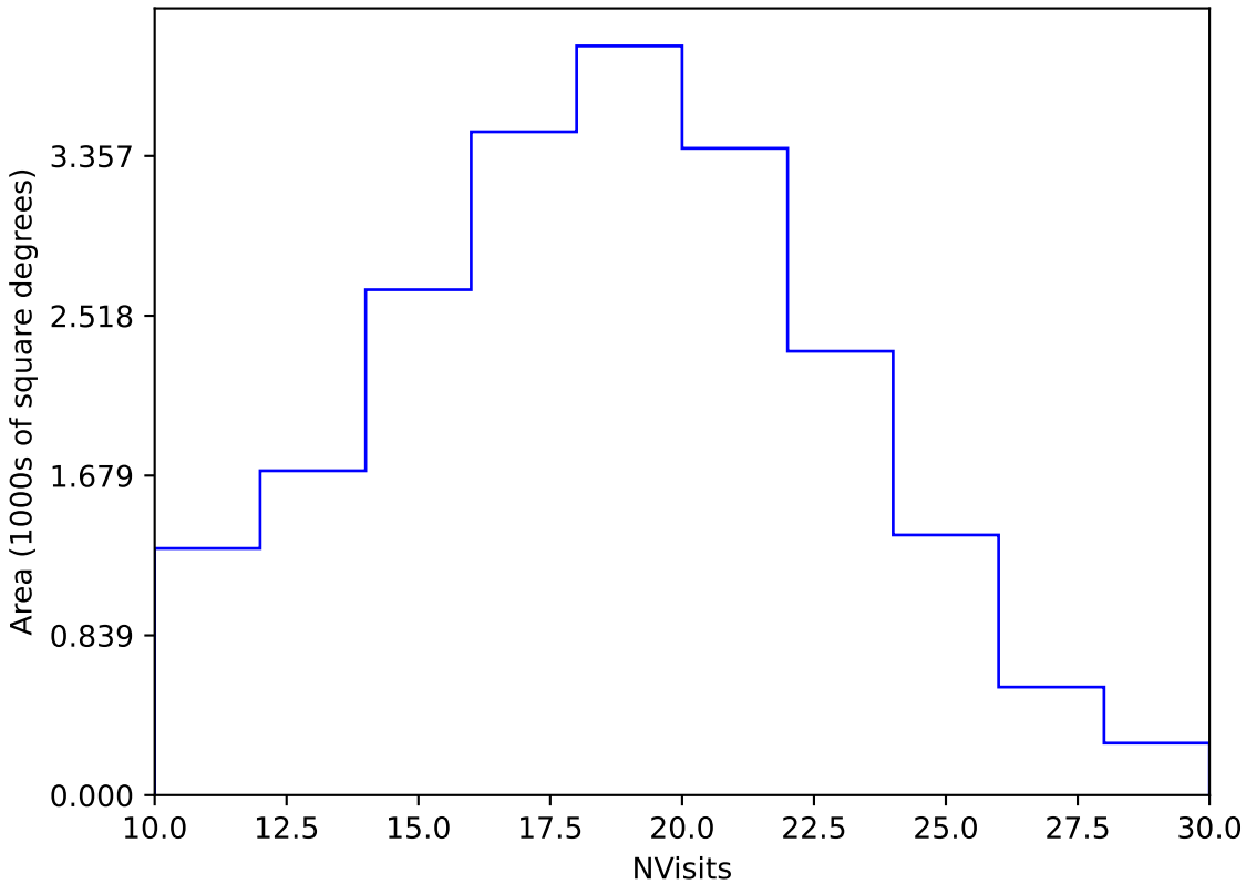
internal_u_expt60_nscale1.2v3.4_10yrs Yr 1 y band: NVisits
