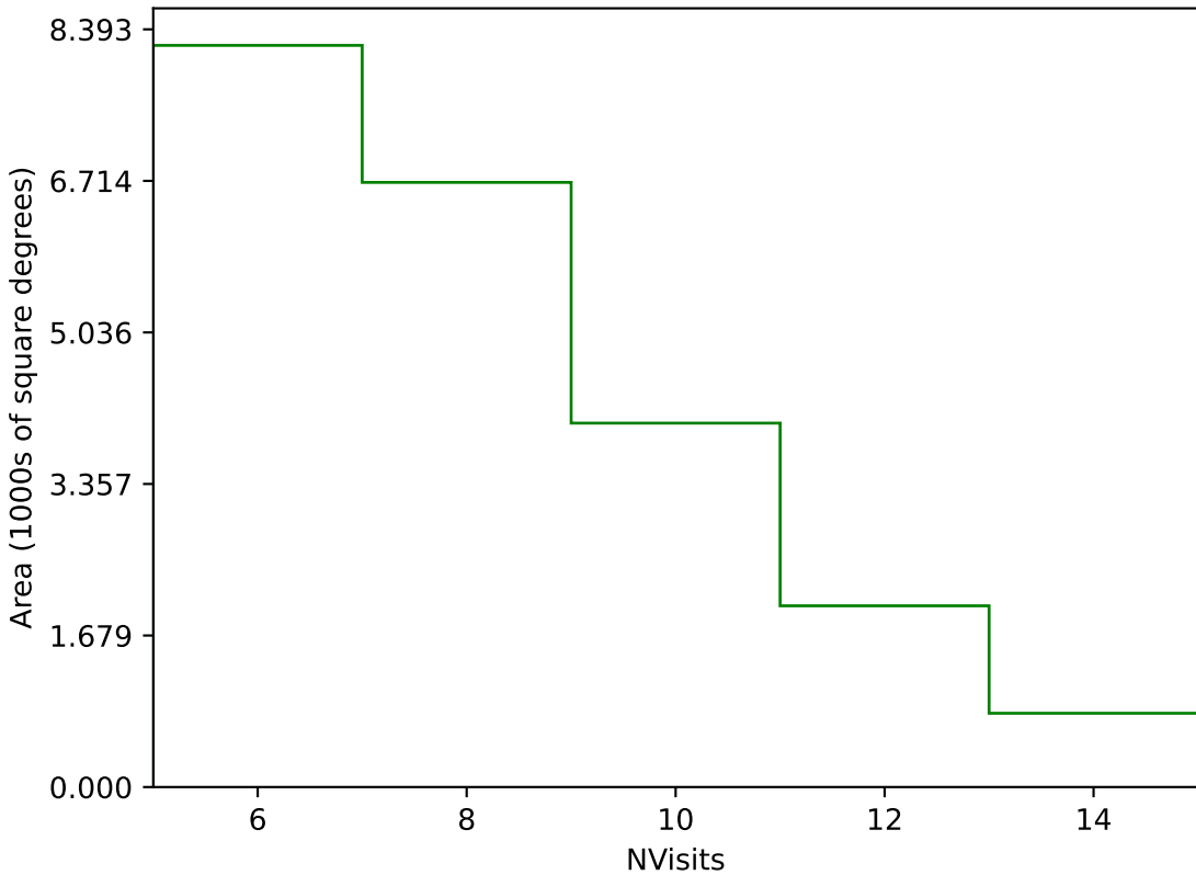
internal_u_expt60_nscale1.2v3.4_10yrs Yr 1 g band: NVisits
