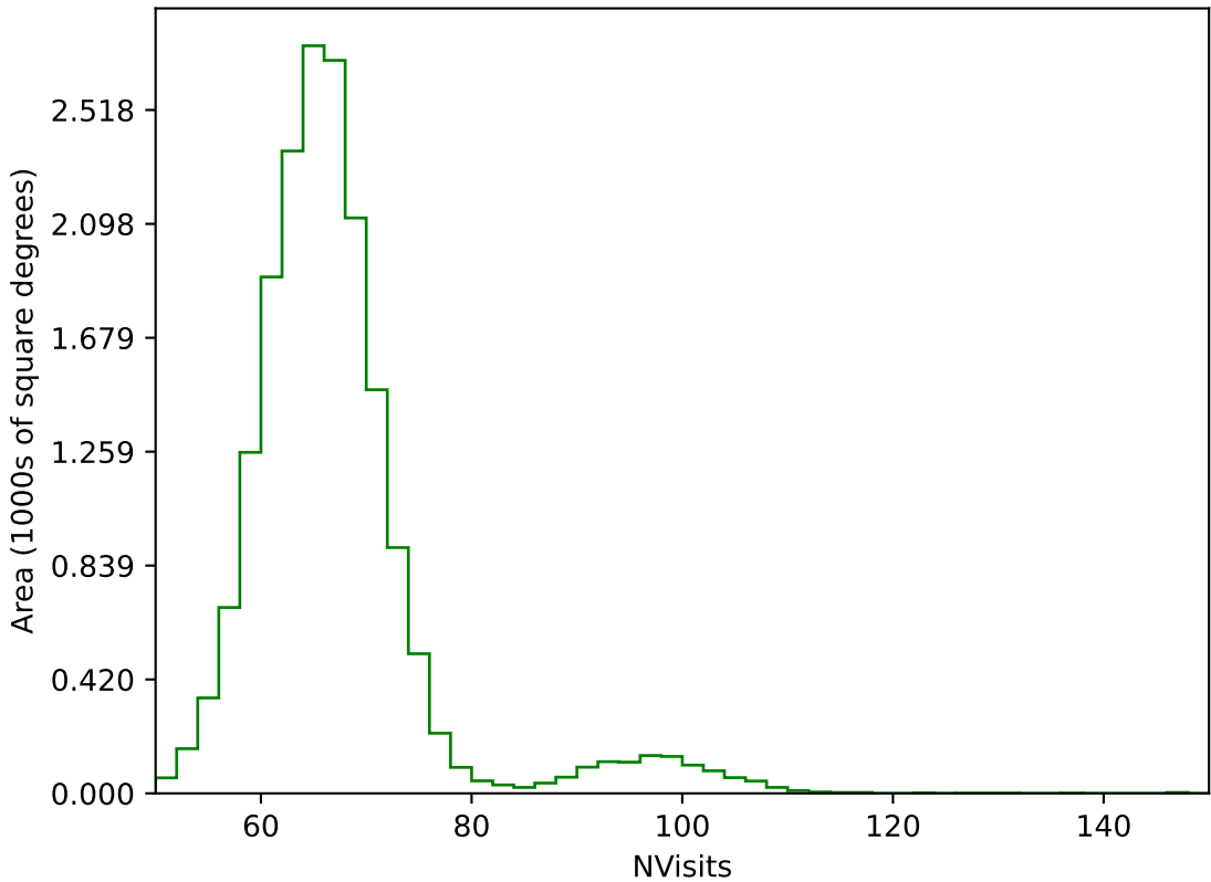
internal_u_expt60_nscale1.2v3.4_10yrs WFD g band: NVisits
