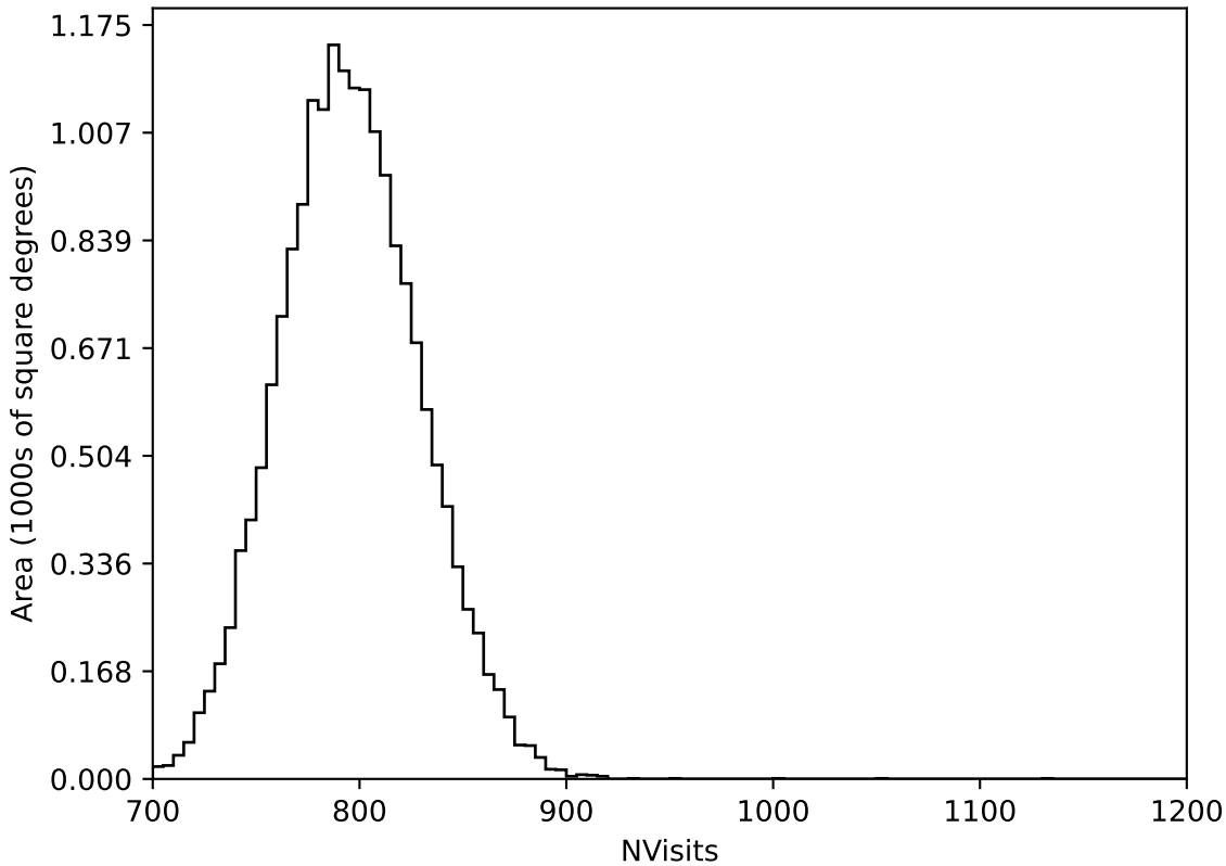
internal_u_expt60_nscale1.2v3.4_10yrs WFD all bands: NVisits
