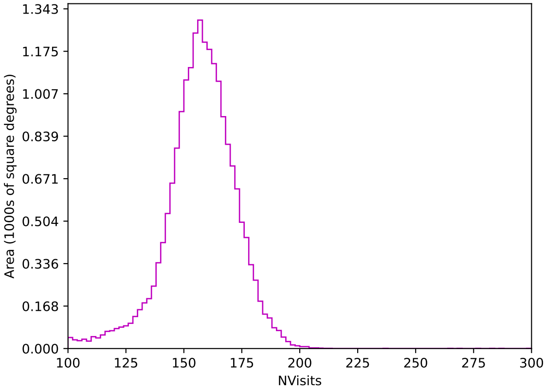
internal_u_expt60_nscale1.2v3.4_10yrs All sky z band: NVisits
