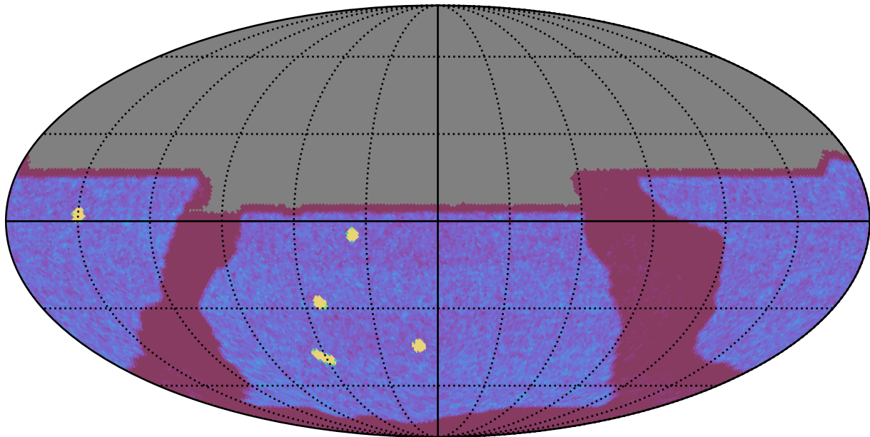
internal_u_expt60_nscale1.2v3.4_10yrs All sky y band: NVisits
