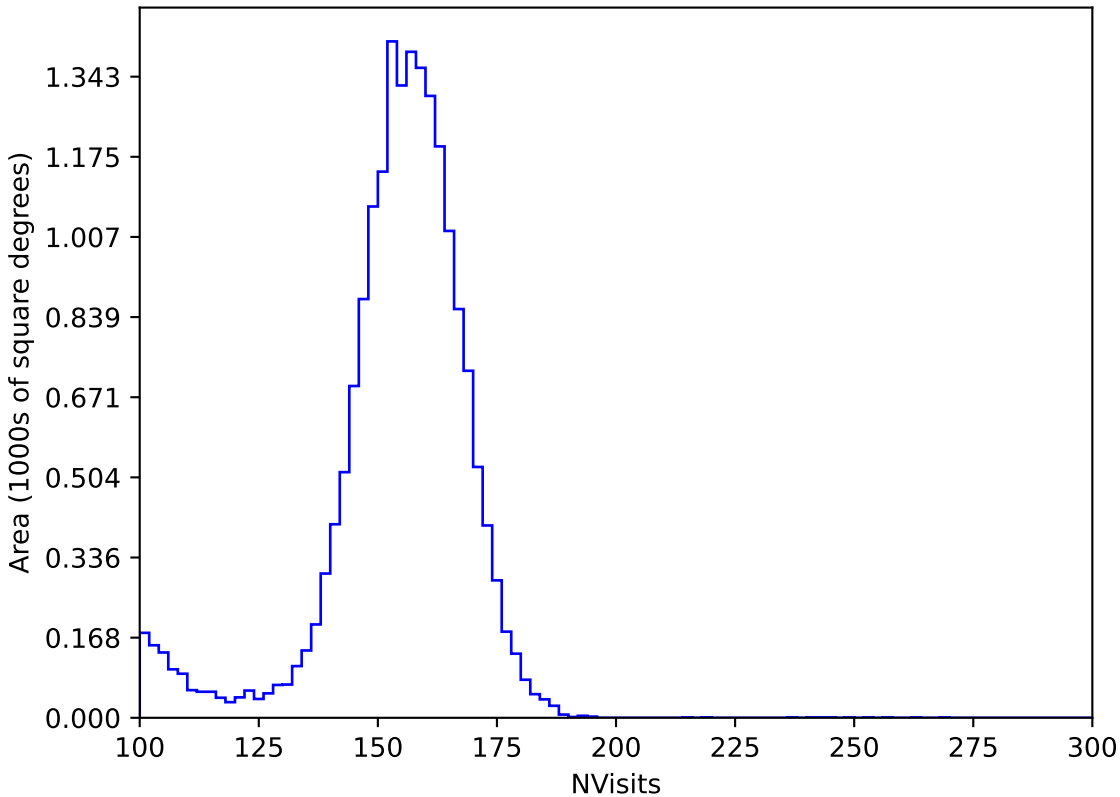
internal_u_expt60_nscale1.2v3.4_10yrs All sky y band: NVisits
