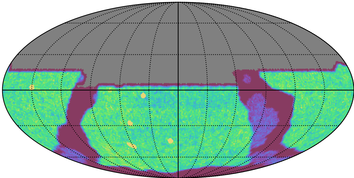
internal_u_expt60_nscale1.2v3.4_10yrs All sky u band: NVisits
