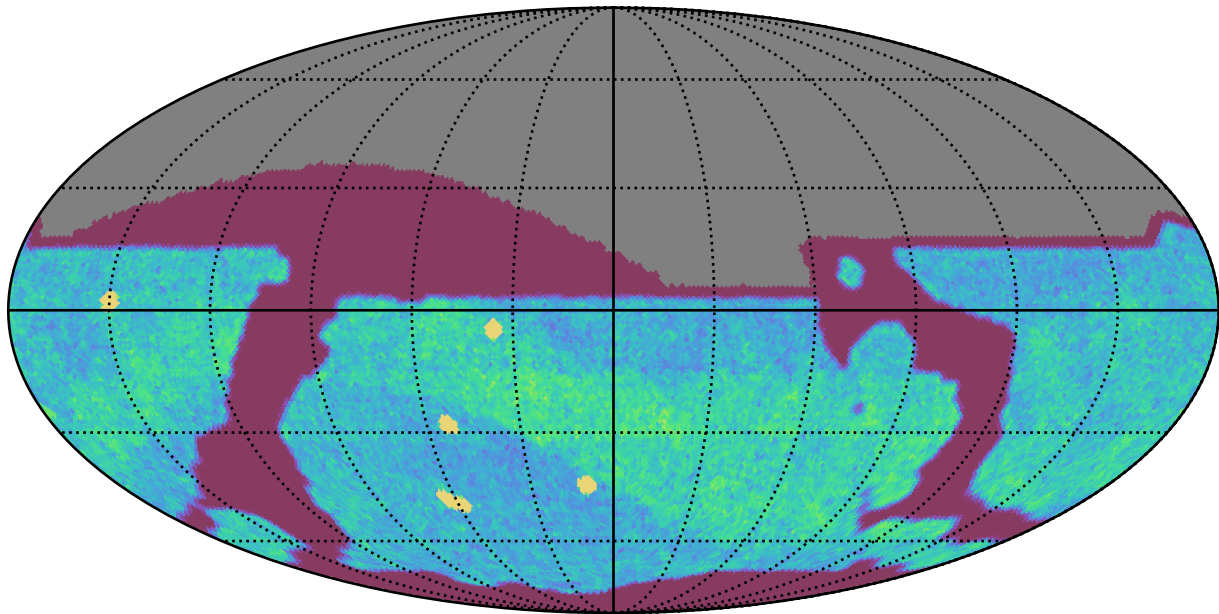
internal_u_expt60_nscale1.2v3.4_10yrs All sky i band: NVisits
