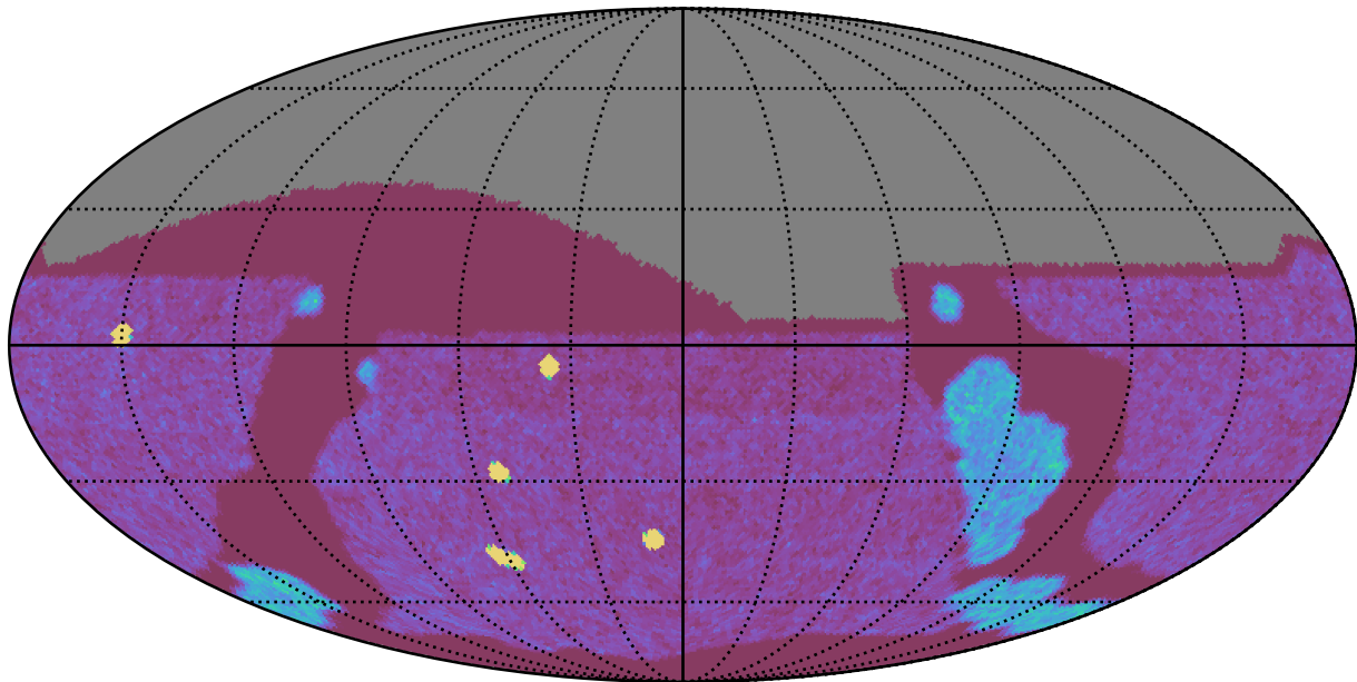
internal_u_expt60_nscale1.2v3.4_10yrs All sky g band: NVisits
