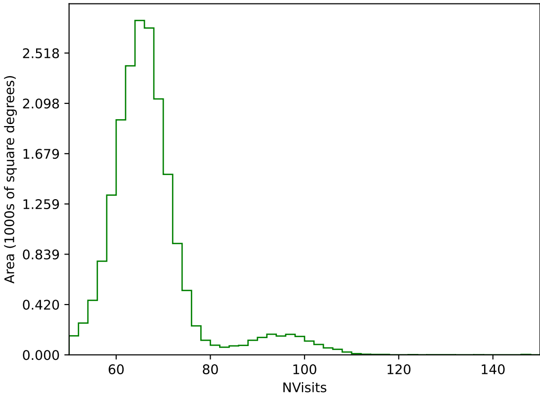
internal_u_expt60_nscale1.2v3.4_10yrs All sky g band: NVisits
