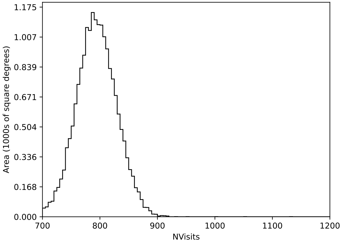
internal_u_expt60_nscale1.2v3.4_10yrs All sky all bands: NVisits
