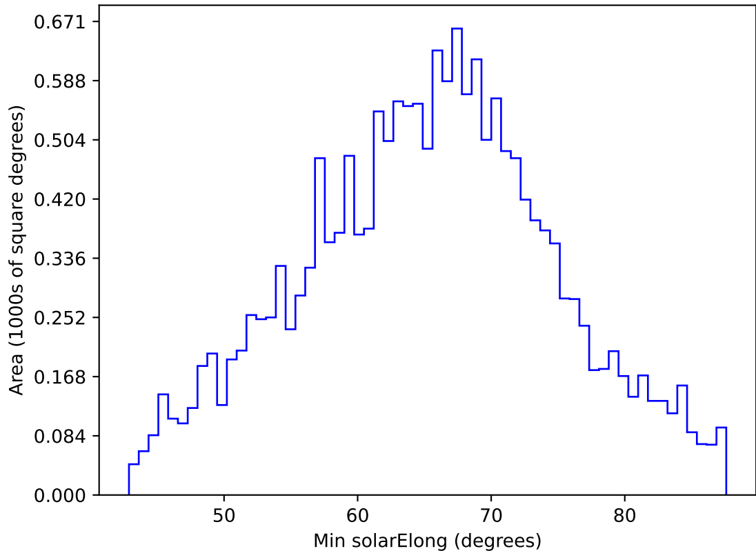
internal_u_expt60_nscale1.2v3.4_10yrs WFD y band: Min solarElong
