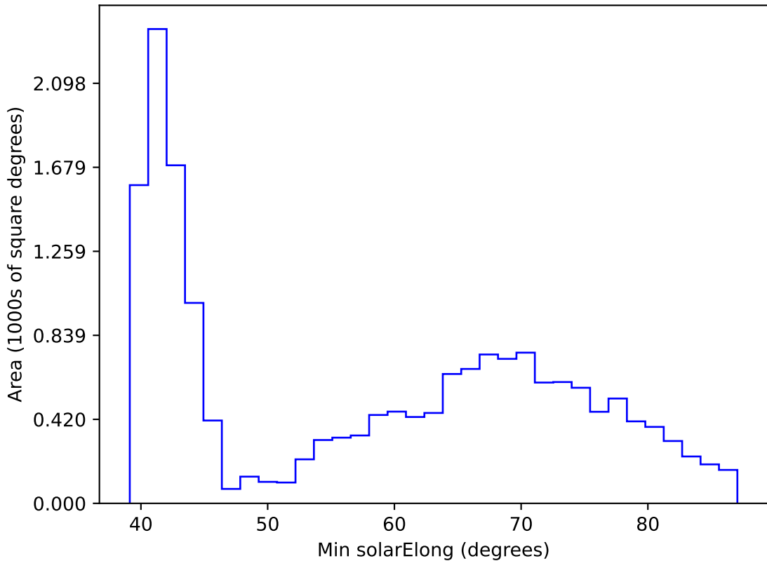
internal_u_expt60_nscale1.2v3.4_10yrs WFD r band: Min solarElong
